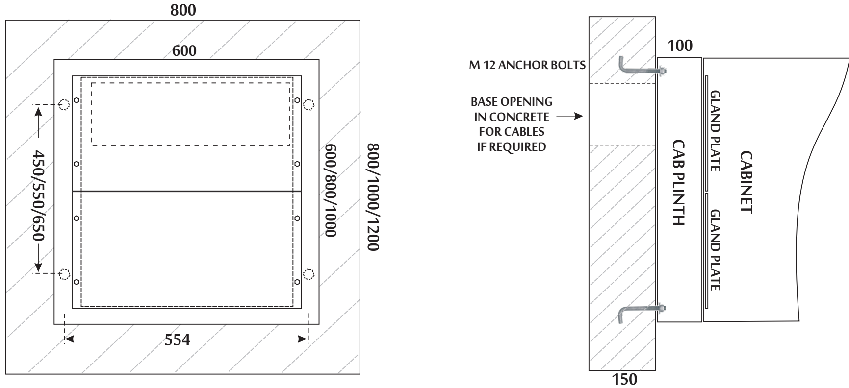
CONCRETE PLINTH DETAILS
